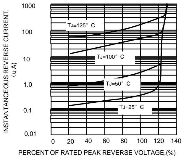
FIG.5-TYPICAL REVERSE CHARACTERISTICS
