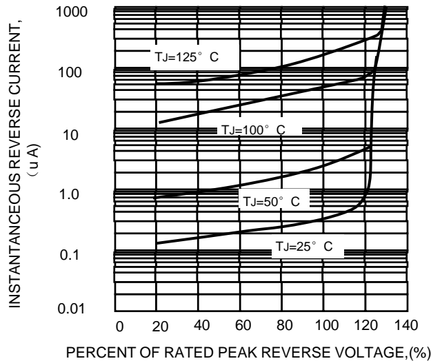
PERCENT OF RATED PEAK REVERSE VOLTAGE, (%) CHARACTERISTICS
