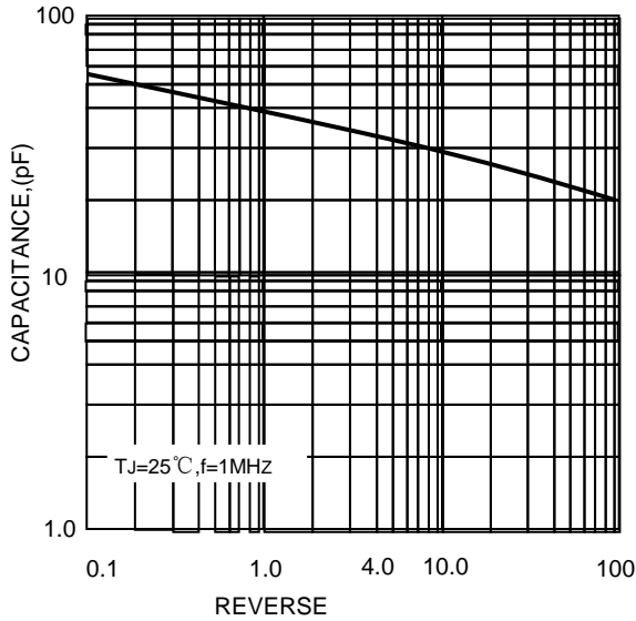
FIG.3-TYPICAL JUNCTION
