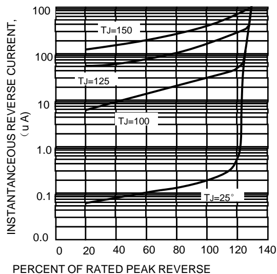
FIG.5-TYPICAL REVERSE
