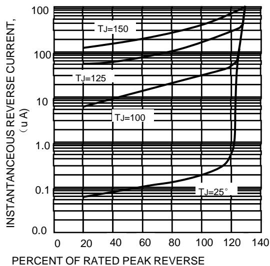
FIG.5-TYPICAL REVERSE CHARACTERISTICS
