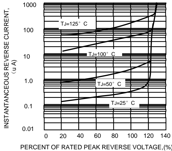
FIG.5-TYPICAL REVERSE CHARACTERISTICS
