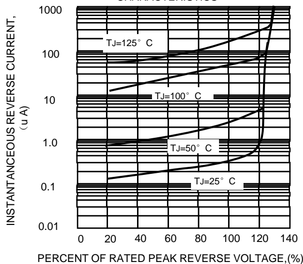
FIG.5-TYPICAL REVERSE CHARACTERISTICS
