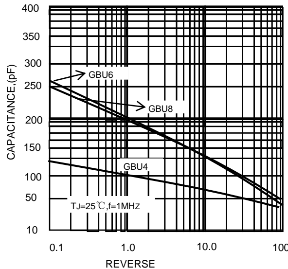
FIG.5-TYPICAL JUNCTION
