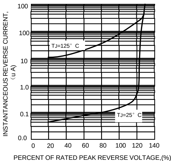
FIG.5-TYPICAL REVERSE CHARACTERISTICS
