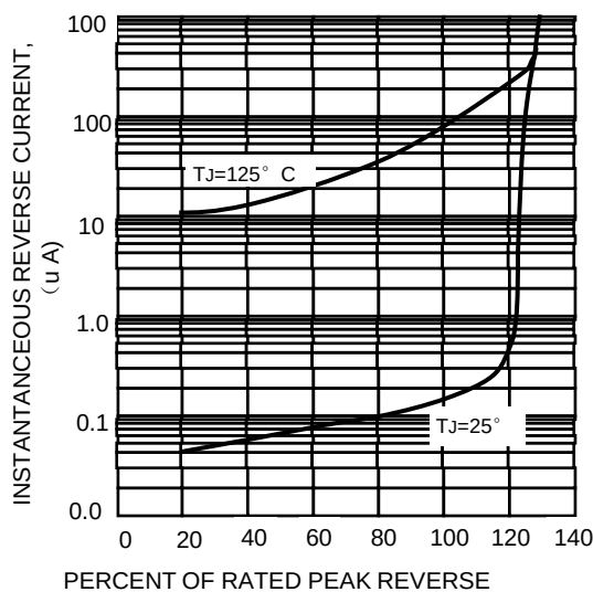
FIG.5-TYPICAL REVERSE
